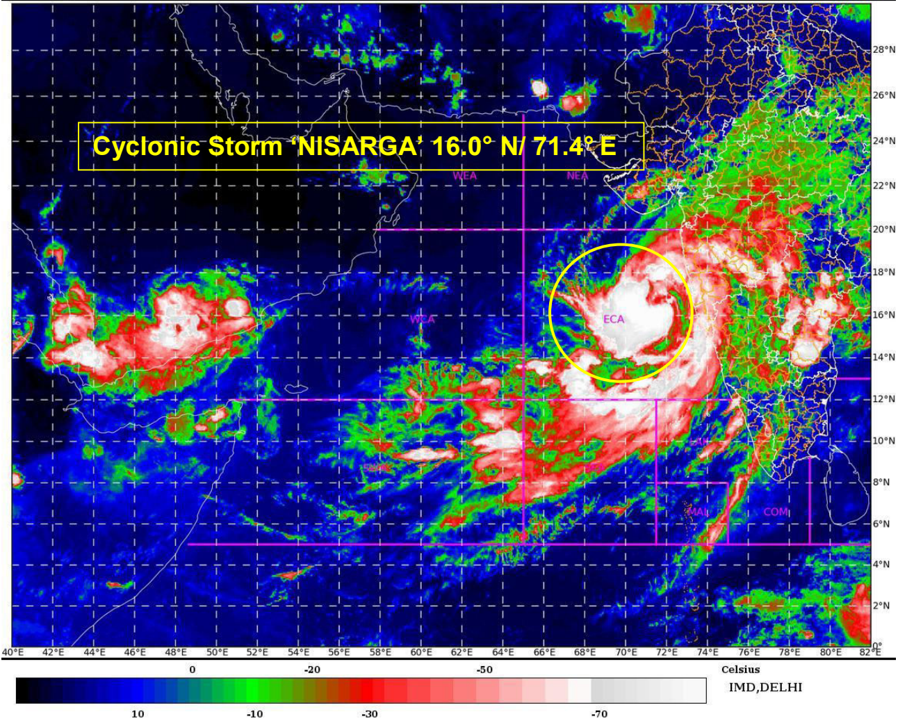
Legend: ECA- east-Central Arabian Sea
